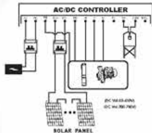
Controller
